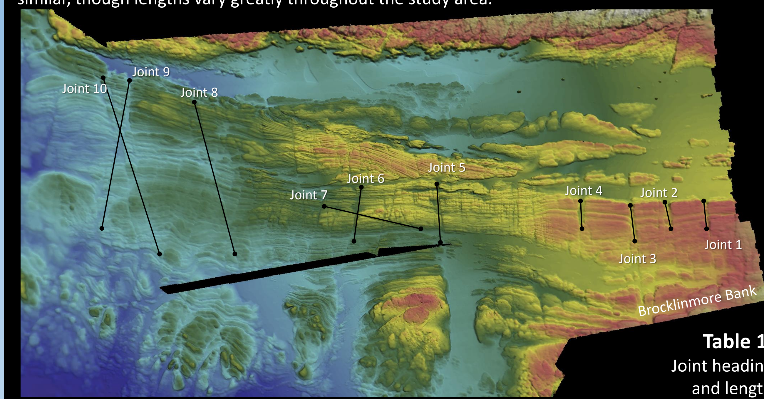
Figure 7. Headings for Joints 1-10 were measured in Google Earth (Table 1). Joint headings are similar, though lengths vary greatly throughout the study area.
